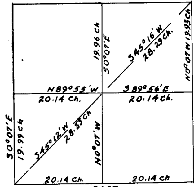
Diagram of SW 1/4 Sec. 32 T5N, R29E, W.M. in accordance with G.L.O. Survey by Erickson in 1906. On file in Recorder's Office, Umatilla County This survey is basis for bearings and Section dimensions applicable to Survey of Eves property
