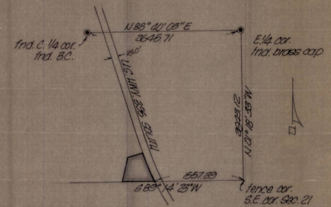
G.E. 1/4 Section 21, T2N, R32E, W.M. 1" = 1000'
