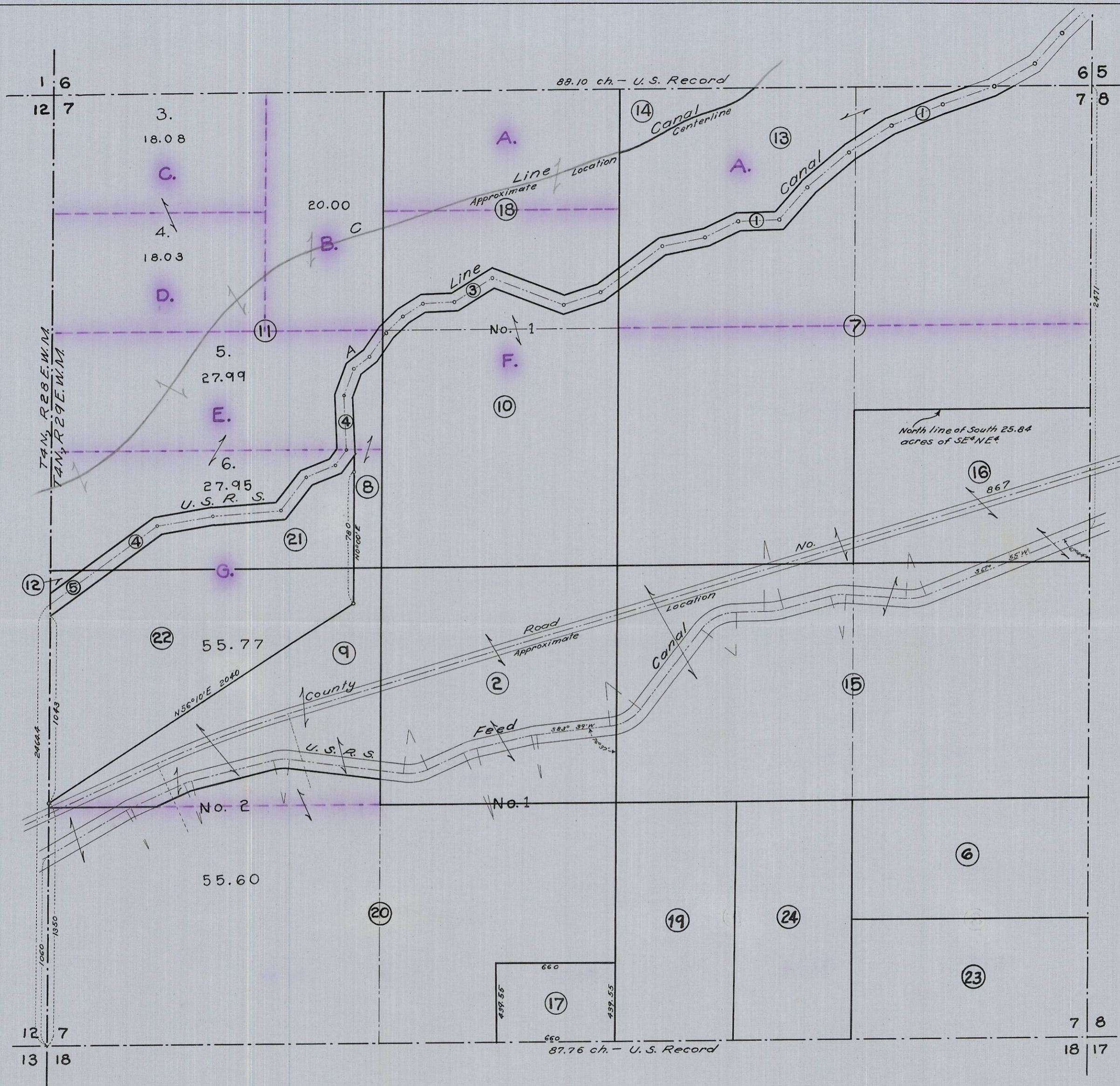
Section 7 T4N., R29E.W.M. Scale 1 inch = 500 feet.
